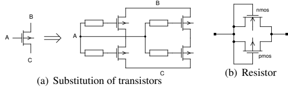
Figure 3. New defect tolerance method
