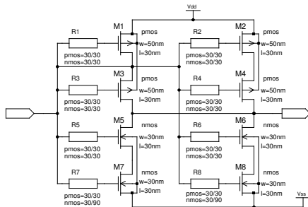
Figure 4. Defect tolerant inverter
