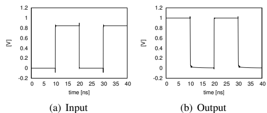
Figure 6. Simulation of inverter in figure 4 (M7 gate to V_{ss} shorted)
