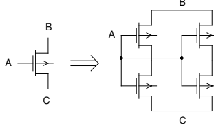
Figure 1. Series and parallel technique
