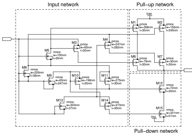
Figure 2. Evolved defect tolerant inverter
