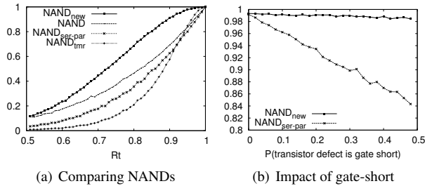
Figure 7. Monte Carlo reliability simulations
