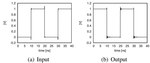
Figure 5. Simulation of inverter in figure 4
